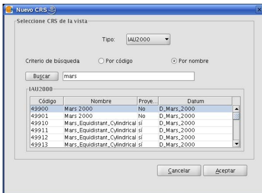
Figure 4. IAU2000 Repository.
