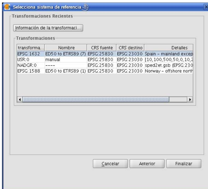
Figure 13. Recent transformations
