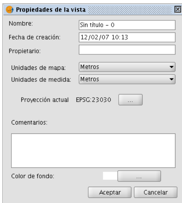
Figure 6. View properties
