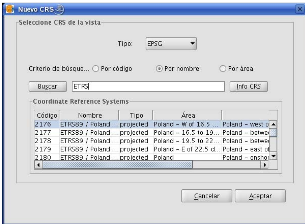
Figure 3: EPSG Repository
